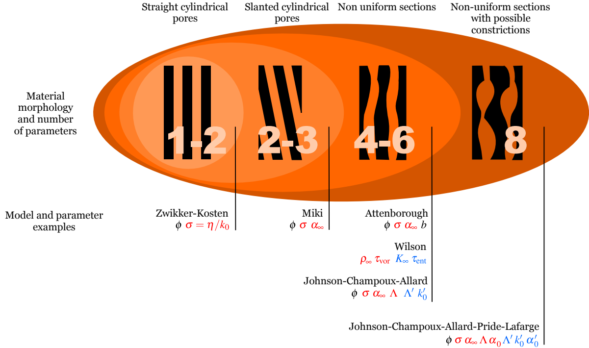
Figure 1: Growing complexity of visco-thermal models used to describe the sound propagation in porous media depending on their pore microstructure. In red: visco-inertial parameters, in blue: thermal parameters.
